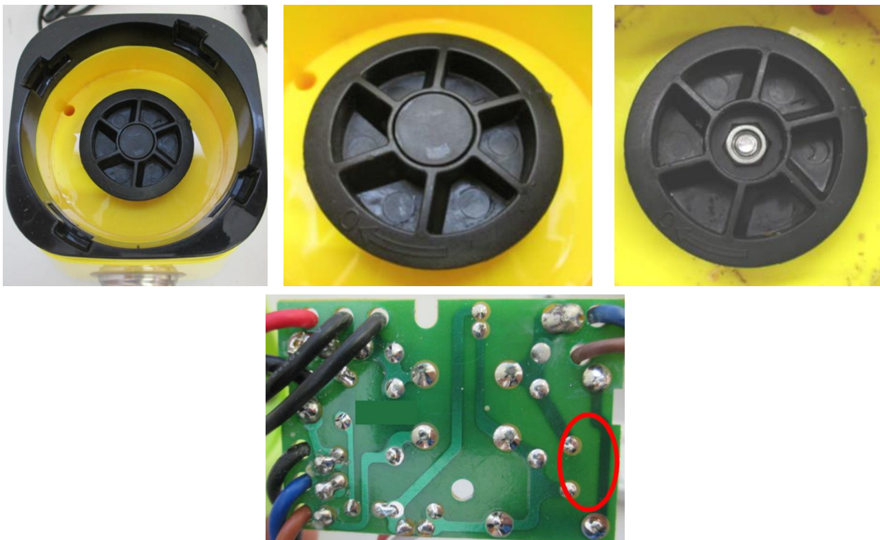
Figure 12 Blender couplings with exposed basic insulation of the motor shaft
