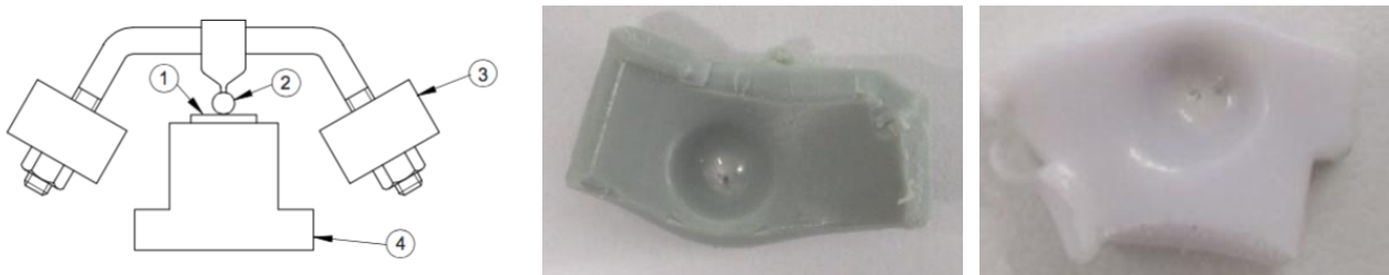
Figure 16 Ball pressure apparatus and indentation in samples exceeding 2 mm in diameter
